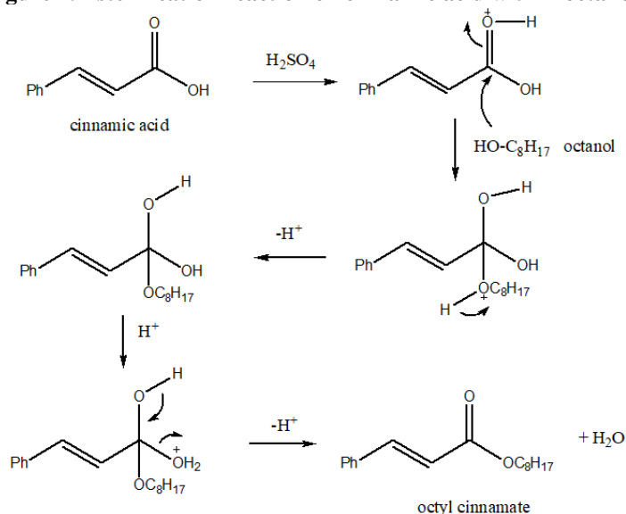
Figure 2. Mechanism of esterification cinnamic acids and octanol
