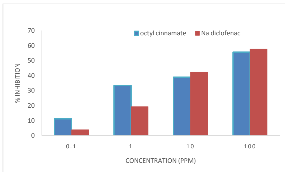
Figure 6. curve % inhibition inhibisidiflofenac sodium dan octil cinnamate
