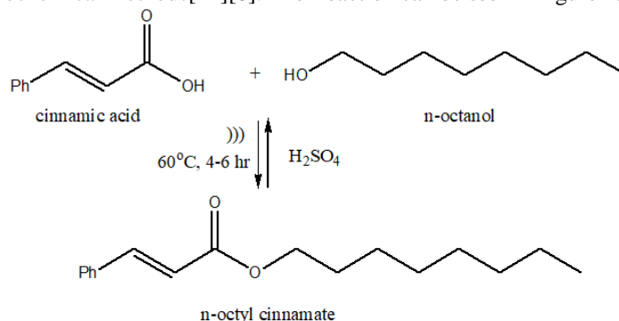
Figure 1. Esterification reaction on cinnamic acid with n-octanol
