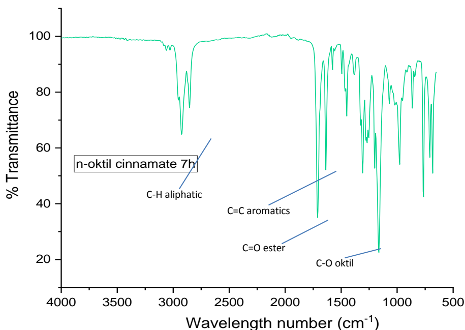
Figure 3. Spectrum FTIR from n-octyl cinnamate
