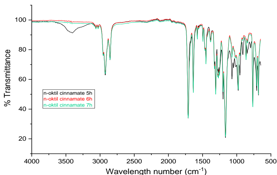
Figure 4. Overlays FTIR n-octyl cinnamate 5,6,dan 7 hours
