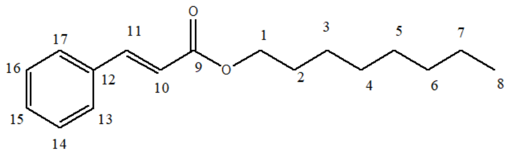
Figure 5. Structure n-octyl cinnamate
