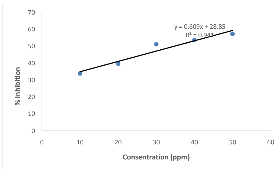
Figure 6. Linear Regression Curve for n-octyl cinnamate
