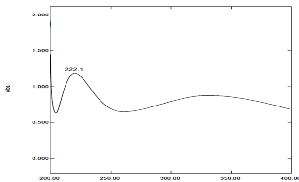
Figure 2: uv spectrum of leniolisib
