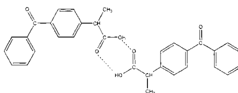
Fig. 4. Dimeric form of crystalline ketoprofen.
