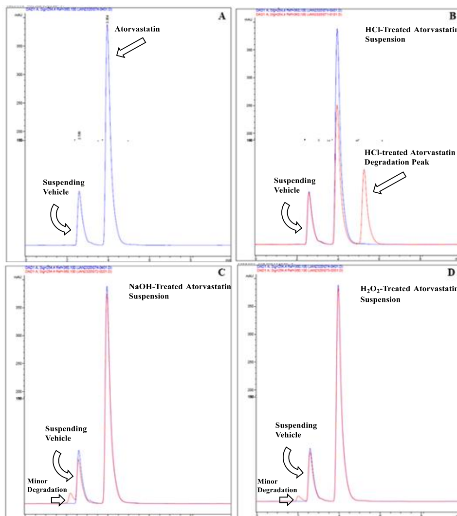
Figure no 2: Forced Degradation of Atorvastatin. (A) Time 0 Chromatogram. Using an equivalent amount of Oral-Plus and Ora-Sweet, atorvastatin had a consistent retention time of 3.9 minutes and the suspending vehicle mixture had a retention time of 2.5 minutes. Freshly prepared atorvastatin suspension was treated with an equivalent amount of 1 M HCl (B), 1 M NaOH (C), and 3% H 2 O 2 (D) for 48 hours at room temperature. Treatment with acid (B) resulted in significant degradation of atorvastatin as demonstrated by a decrease in the parent molecule peak height and AUC relative to untreated samples (blue) and the appearance of a new degradation peak (red overlay) which is shown with a retention time of 5 minutes. Treatment with base (C) or peroxide (D) had little impact on the overall stability of atorvastatin.
